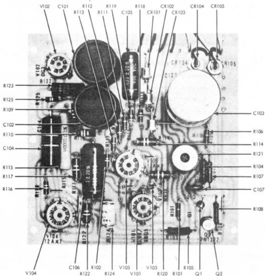
Figure 5-3. REFERENCE SUPPLY BOARD ASSEMBLY
